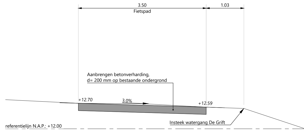
PRINCIPLEPROFIEL F-F
